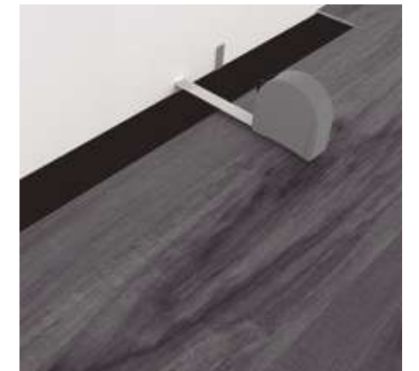
Step 10: Last row. The Minimum width of the last plank should be NOT LESS than 2" wide. Put a spacer before measuring Cut the panels lengthwise and glue the short ends.
