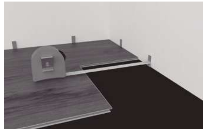
Step 4: At the end of the first row, put a spacer 3/8" (9,525mm) to the wall and measure the length of the last plank to fit.
