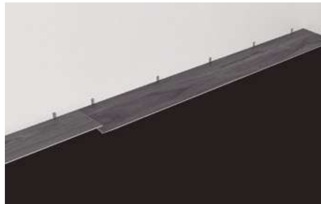
Step 3: Fold the panel down in a single action movement. Afterwards press down or slightly tap down at the short end just installed till it clicks.
