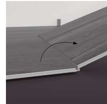
Step 8a: Second plank, second row. Place the panel at an angle into the groove of the previous row making sure that the end of the panel is tight/flush to the short end of the previous panel.
