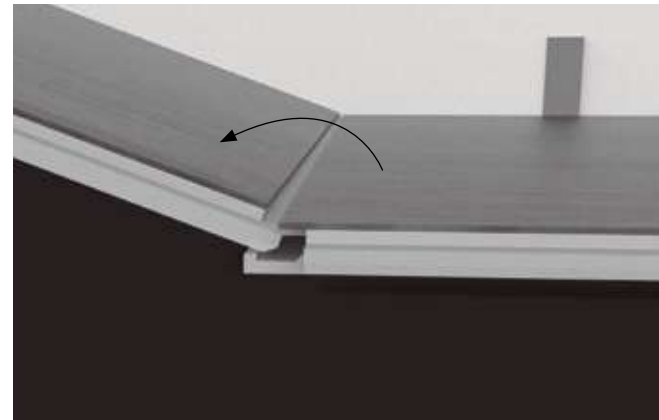
Step 2: Second plank, first row. Place this plank gently and tight to the short end of the first one.
