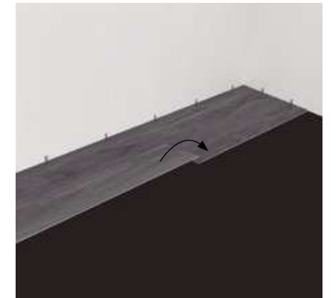
Step 8b: Fold the panel down in a single action movement with a slight press to the left to the short end of the previous panel. Again, using the tapping block tap it against the long end into the previous row.
